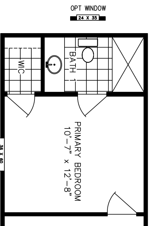
OPT. BATH 1 LAYOUT W / 60" SHOWER
